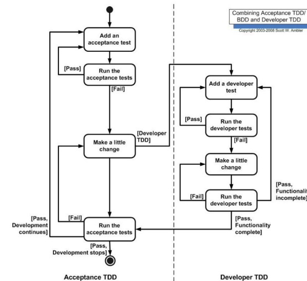
Figure 2 TDD cycle in agile modern driven development
